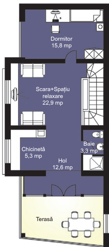
PLAN MANSARDĂ
